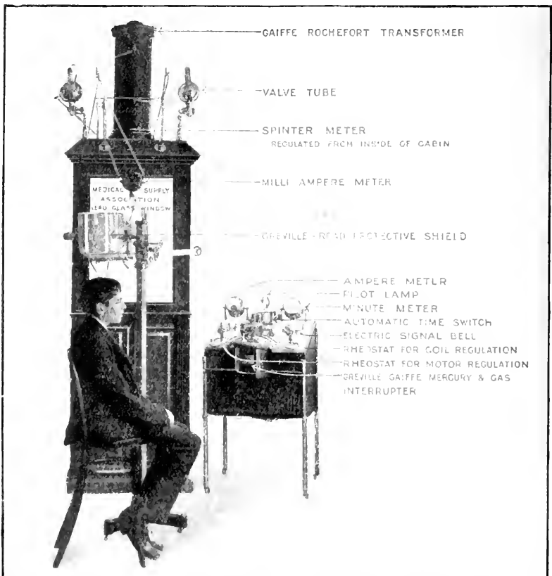
FIG. 195.—A convenient arrangement of apparatus for therapeutic work.
